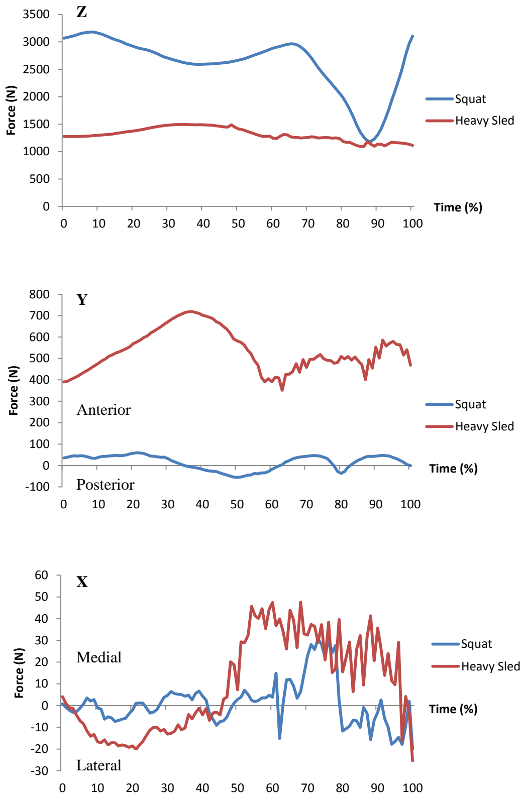
Figure 5: Group Mean Vertical (Top), Anterior/Posterior (Middle) and Medial/Lateral (Bottom) Force-Time Curves (Normalised to Percentage of Mean Lift Time) Obtained With a 70% 1-Repetition Maximum Load for the Squat and Sled pull (From the Start of the Concentric Phase to the Point of Maximal Knee Extension)
