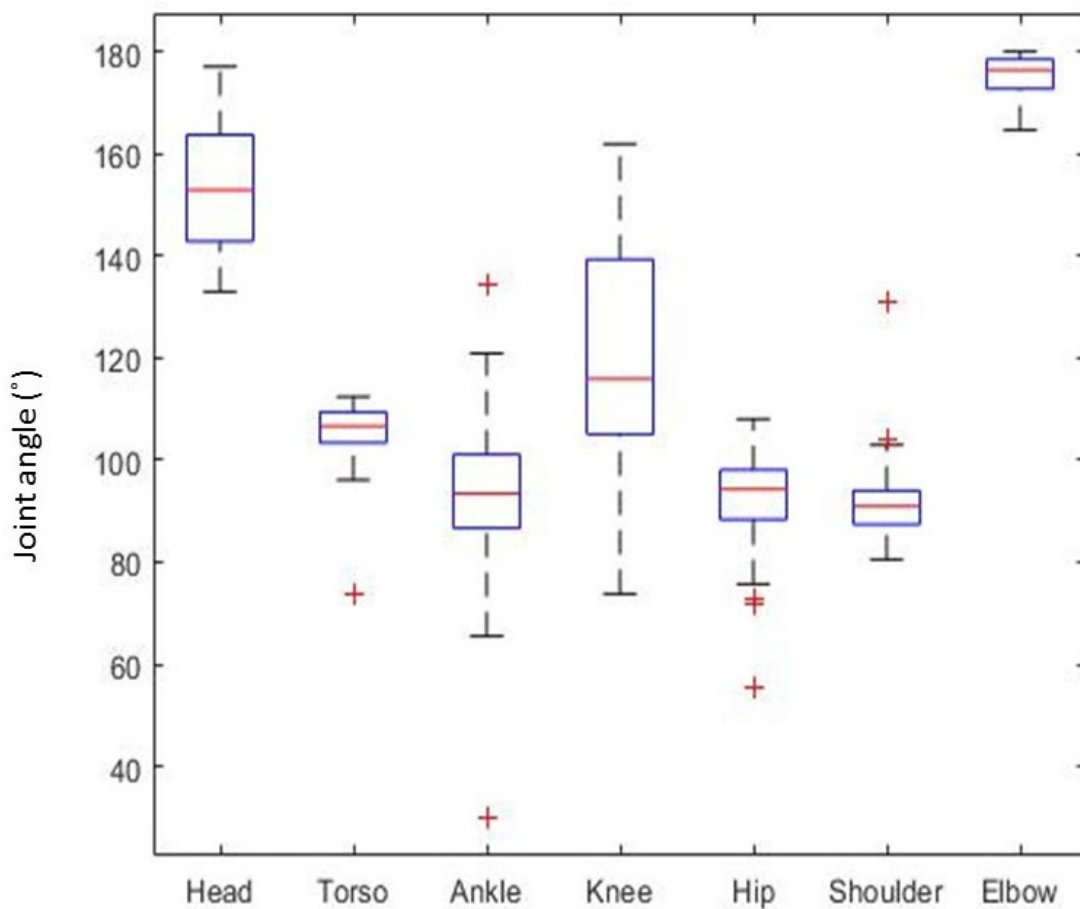
Figure 8-8 Summary of all participants set position, joints vs joint angles
