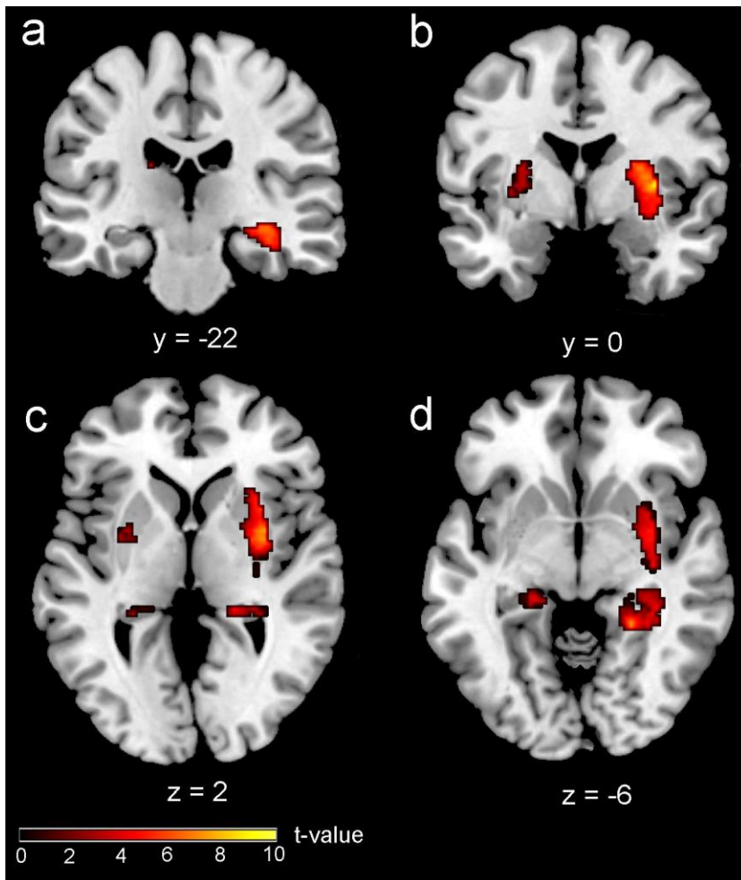
Figure 4. MR brain slices showing mean BOLD activity from the analysis of coordinate minus categorical conditions. (a) Right hippocampus. (b) Left and right dorsal striatum. (c) Bilateral hippocampus and dorsal striatum. (d) Bilateral hippocampus, right parahippocampus and left dorsal striatum.
