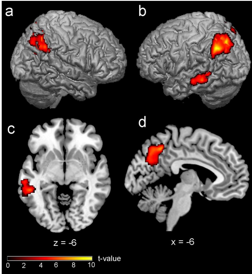
Figure 3. MR brain slices and three-dimensional rendered MR images showing mean BOLD activity from the analysis of categorical minus coordinate conditions. Activation maps are overlaid onto a rendered MNI-normalised template. (a) Right posterior parietal cortex. (b) Left posterior parietal cortex and middle temporal gyrus. (c) Left middle temporal gyrus (d) Medial parietal cortex (precuneus).
