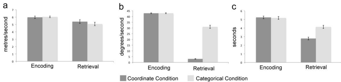
Figure 2. Mean behavioural performance ( \pm 1 standard error) during encoding and retrieval phases of the navigation task, plotted separately for the coordinate and categorical conditions. (a) Speed. (b) Unsigned rotation. (c) Duration.
