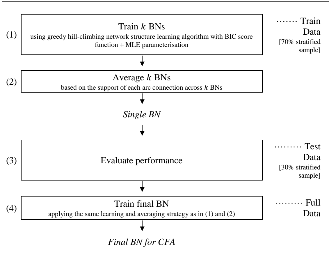
Figure 2. Bayesian network model fitting process.
