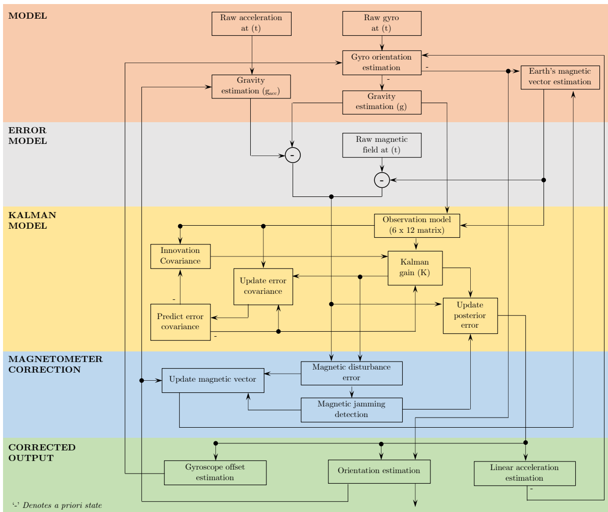
Figure 5.3 Kalman filter approach example (adapted from MEMS Industry Group [167] and The MathWorks Inc. [168]).
